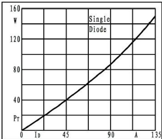
Fig2. Power dissipation
